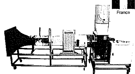
Test bench of an axial fan
