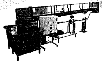
Study of flows in an open channel section
