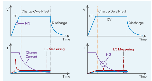
Completed lithium-ion battery insulation anomaly detection
